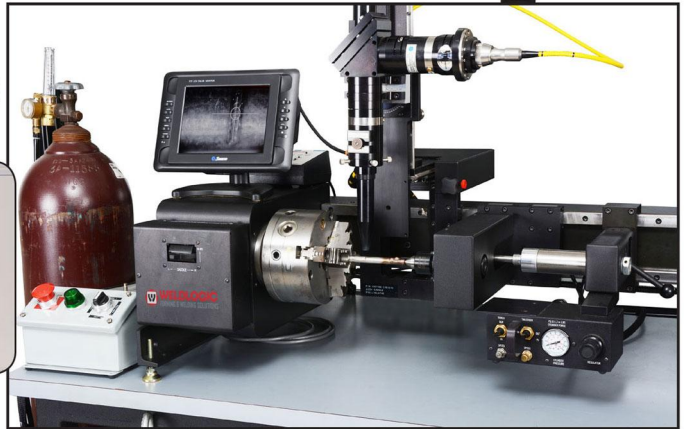
Lathe can be oriented horizontally (as shown) or vertically
